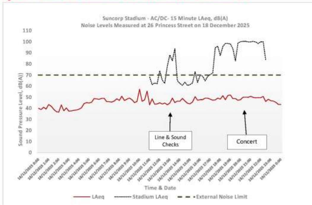
Figure 8: External Noise Measurements - Site 4 – 26 Princess Street on 18 December 2025.
