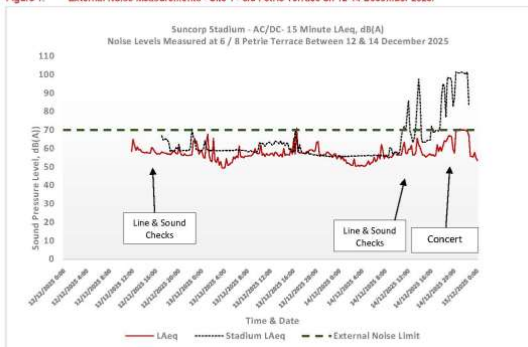
Figure 1: External Noise Measurements - Site 1 - 6/8 Petrie Terrace on 12-14 December 2025.
