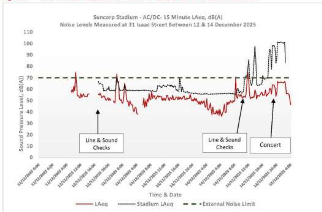
Figure 9: External Noise Measurements - Site 5 – 31 Isaac Street on 12-14 December 2025.
