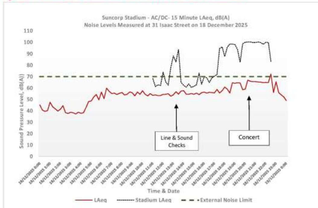
Figure 10: External Noise Measurements - Site 5 – 31 Isaac Street on 18 December 2025.
