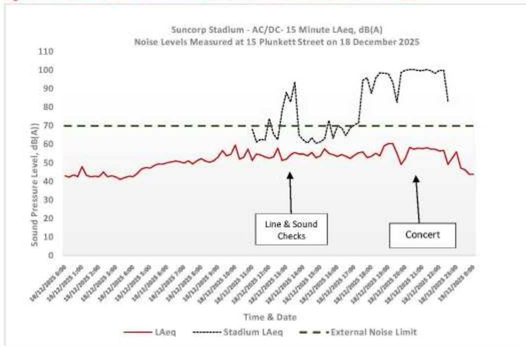
Figure 4: External Noise Measurements - Site 2 – 15 Plunkett Street on 18 December 2025.
