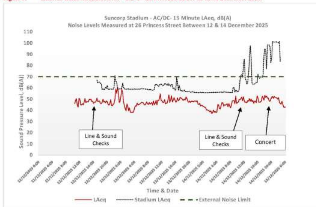
Figure 7: External Noise Measurements - Site 4 – 26 Princess Street on 12-14 December 2025.
