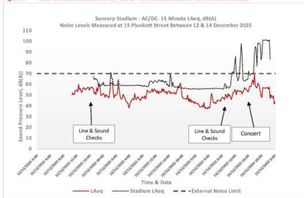
Figure 3: External Noise Measurements - Site 2 - 15 Plunkett Street on 12-14 December 2025.
