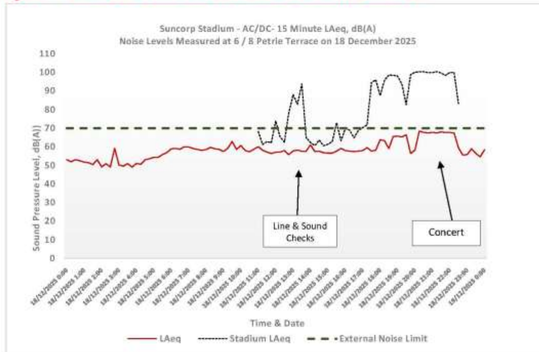
Figure 2: External Noise Measurements - Site 1 - 6/8 Petrie Terrace on 18 December 2025.
