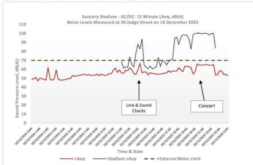
Figure 6: External Noise Measurements - Site 3 – 36 Judge Street on 18 December 2025.
