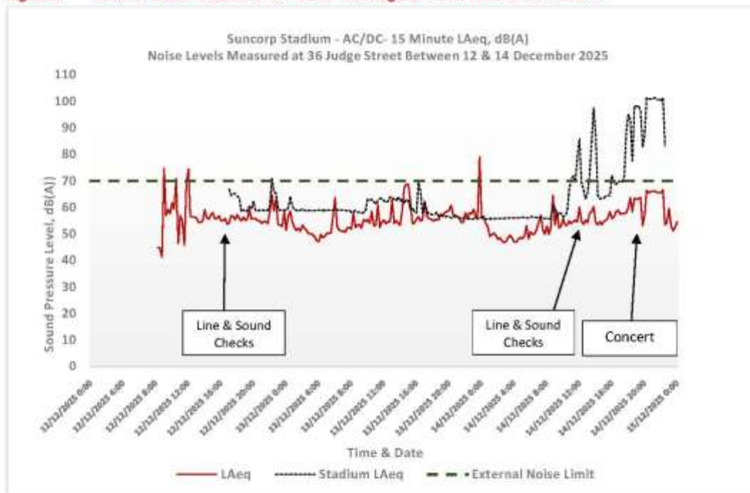
Figure 5: External Noise Measurements - Site 3 – 36 Judge Street on 12-14 December 2025.
